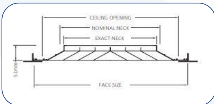
Lay-in Diffuser
